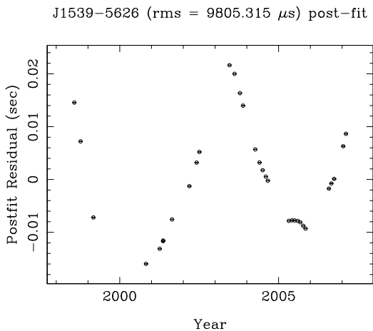
Figure 1: Pulsar timing residuals for PSR J1539–5626 from the young pulsar timing programme, P262.
