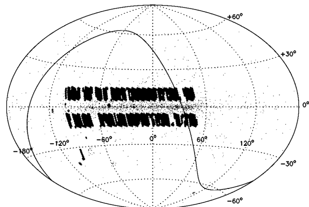
Figure 6: Galactic coordinates for the Swinburne Intermediate Latitude Survey are indicated as bold points. The area of the sky under the solid line is where the Parkes 70 cm was conducted. The small dots are the positions of known pulsars.
