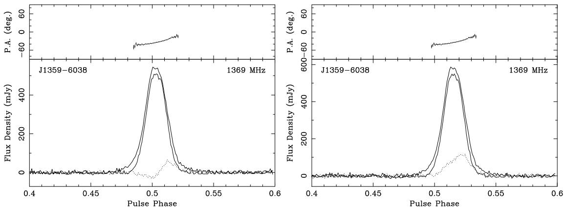
Figure 2: Profile for PSR J1359–6038 obtained by Kelso High School students as part of the PULSE@Parkes project. The profile in the left-hand panel has been calibrated using the standard PAC calibration method. The profile in the right-hand panel has been calibrated with compensation for cross-coupling in the 20 cm feed. The outer solid line represents Stokes I, the inner solid line the linear polarisation (with the position angle shown in the upper panel) and the dotted line shows Stokes V.
